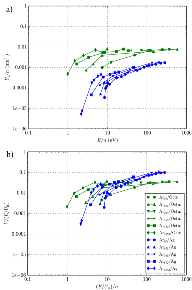
Figure 3. (a) Dependence of Y_v/n in volume units of \text{nm}^3 on E/n for \text{Ar}_n cluster bombardment of octane and Ag(111) surfaces. (b) Same data plotted as Y/(E/U_0) versus (E/U_0)/n .
